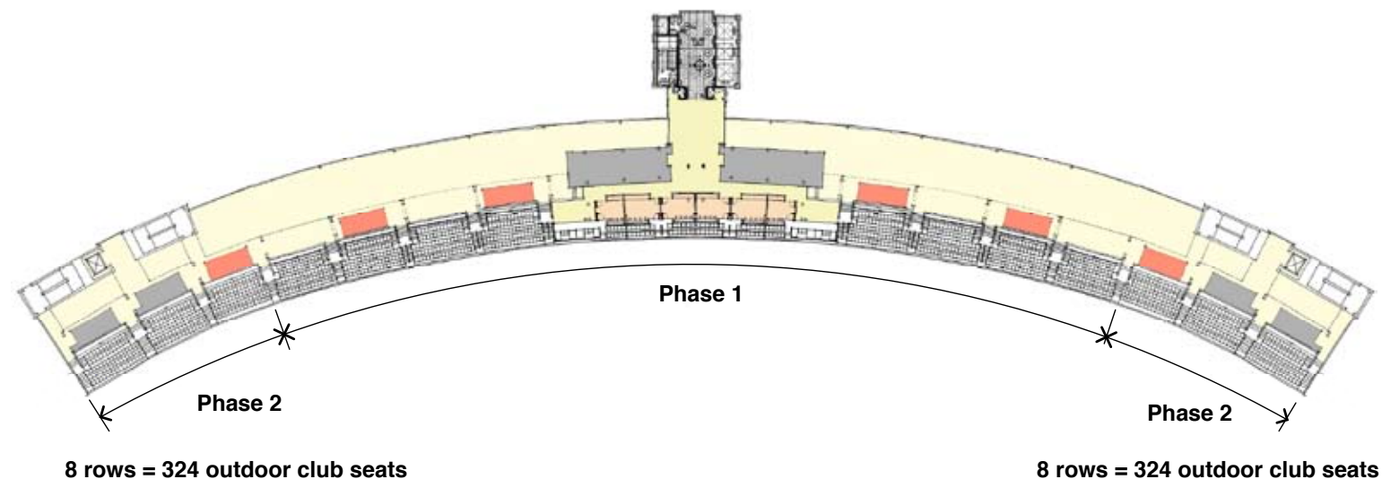
Proposed G Level Plan
